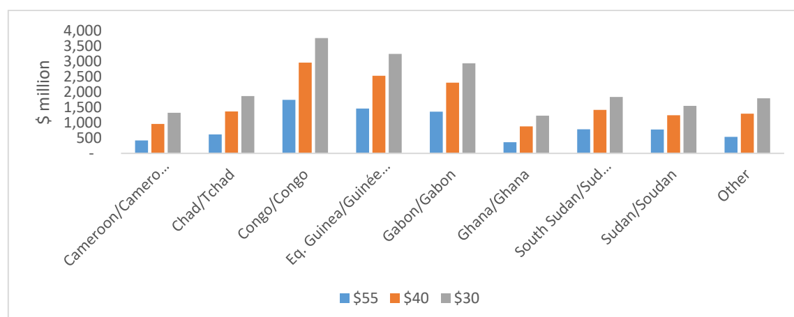
Chart 12b Estimated oil value loss in 2020 compared to 2019, by oil price, other oil producers
