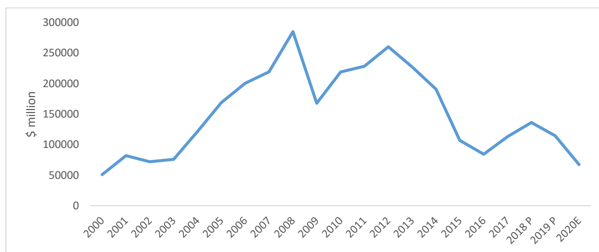
Chart 11: Net crude oil export revenue at constant 2010 prices under a $40 scenario for 2020
