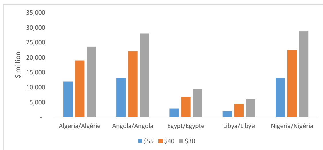
Chart 12b Estimated oil value loss in 2020 compared to 2019, by oil price, other oil producers
