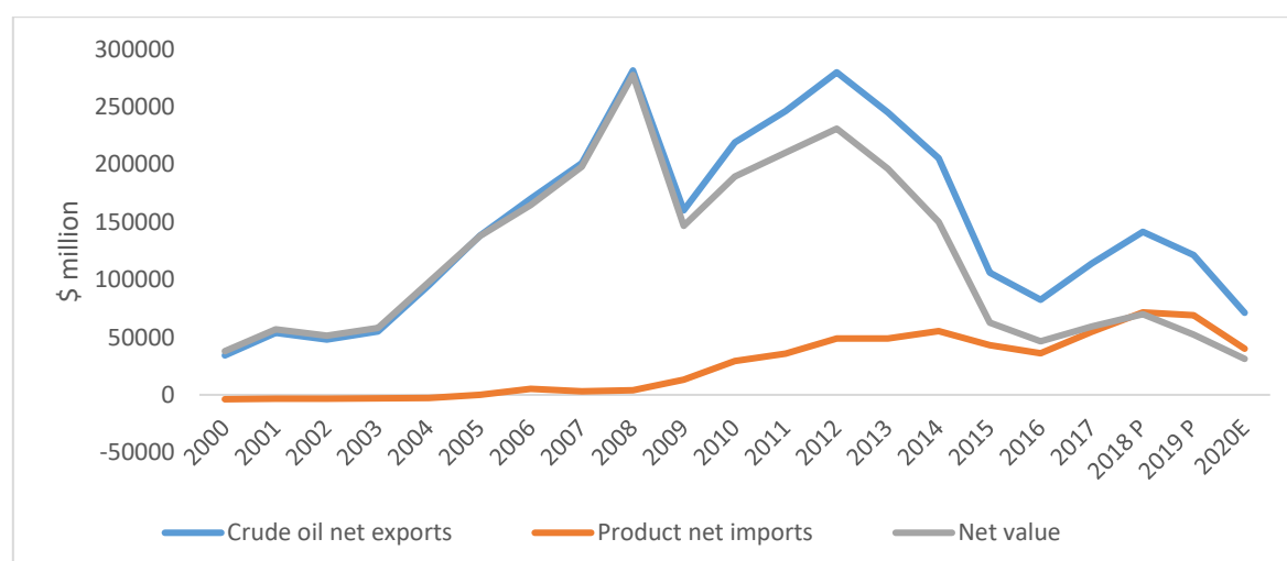
Chart 9: Value of African Oil Trade, including 2020 estimate
