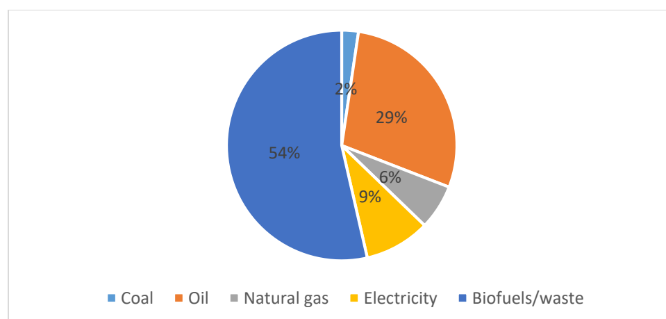
Chart 5: Final Energy Consumption, Africa, 2017
