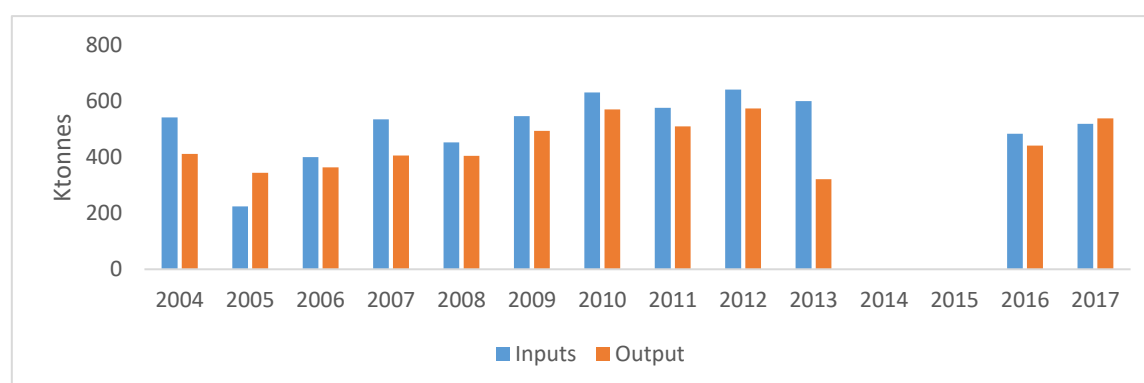
Chart 13: Refinery operations Indeni refinery, Zambia
