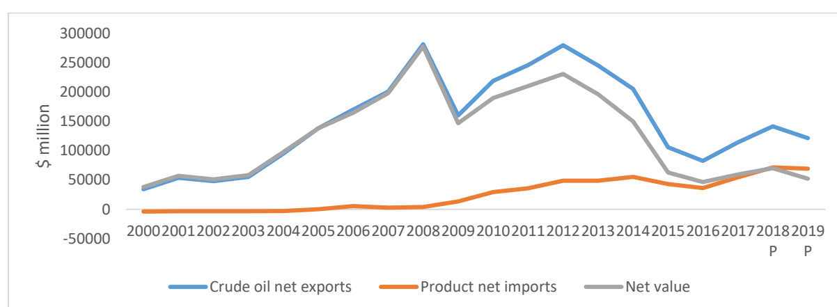
Chart 4 Value of African Oil Trade
